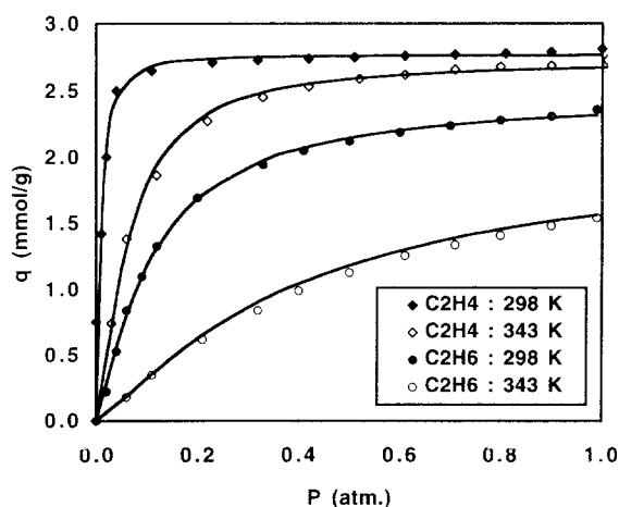
Figure 2. Equilibrium \text{C}_2\text{H}_4 and \text{C}_2\text{H}_6 isotherms on zeolite 4A at 25° and 70°C.
